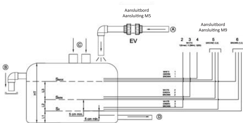
Installatieschema buffertank.
